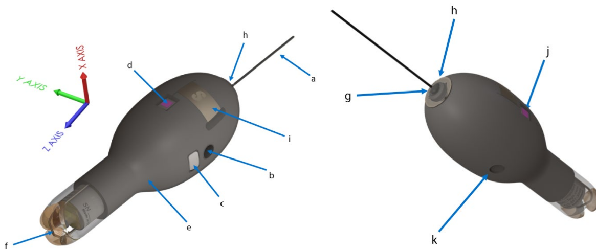
Figures 2 & 3—sPAT tag showing: (a) Argos antenna, (b) temperature sensor, (c) communications port with plug, (d) light sensor (1 of 2), (e) float, (f) release pin, (g) LED light, (h) wet/dry sensor, (i) ground plate, (j) light sensor (2 of 2), and (k) pressure sensor.
